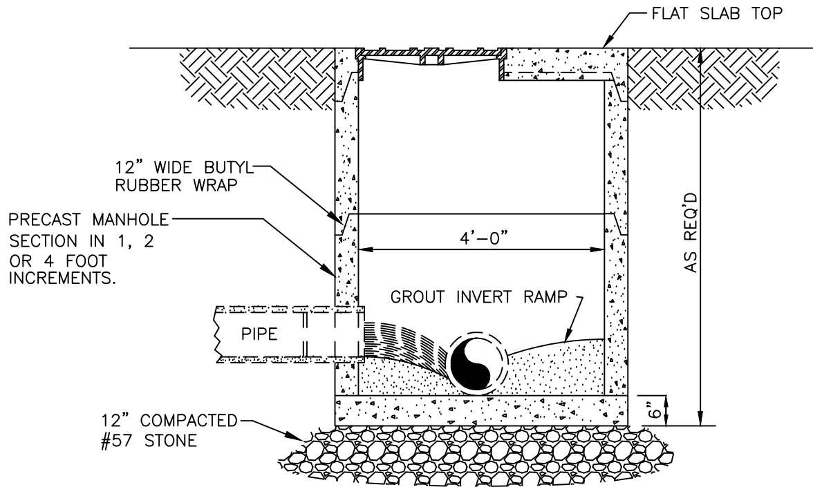
SHALLOW MANHOLE
