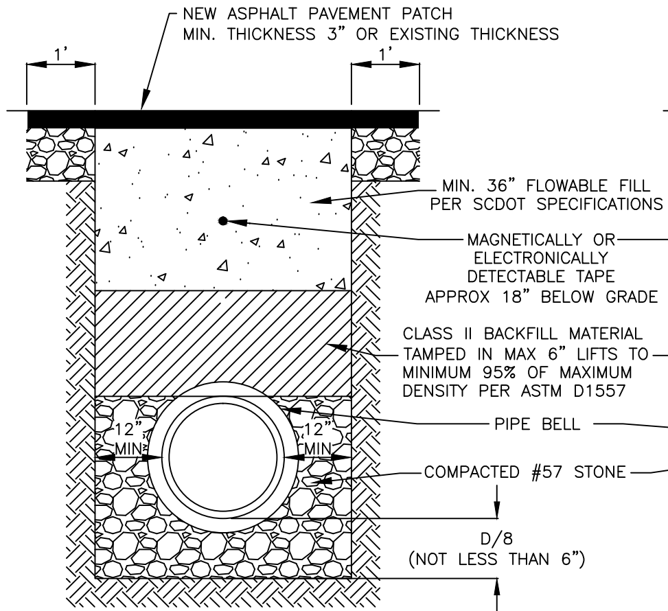
ROAD PAVEMENT CUT DETAIL
