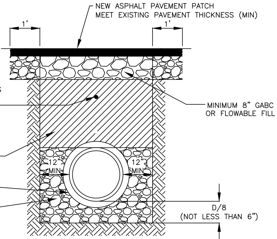
PAVEMENT CUT DETAIL OTHER PAVED AREAS
